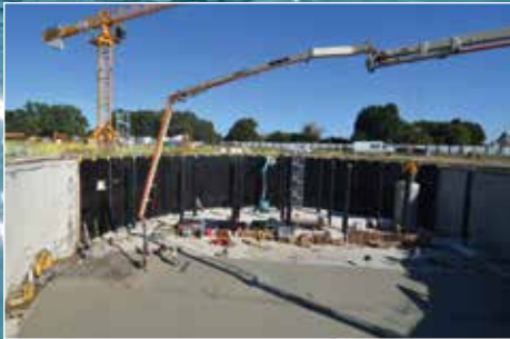
CONCRETE PROTECTION LINING TO PREVENT CONCRETE DETERIORATION ON INTAKE/DISCHARGE CHAMBERS
